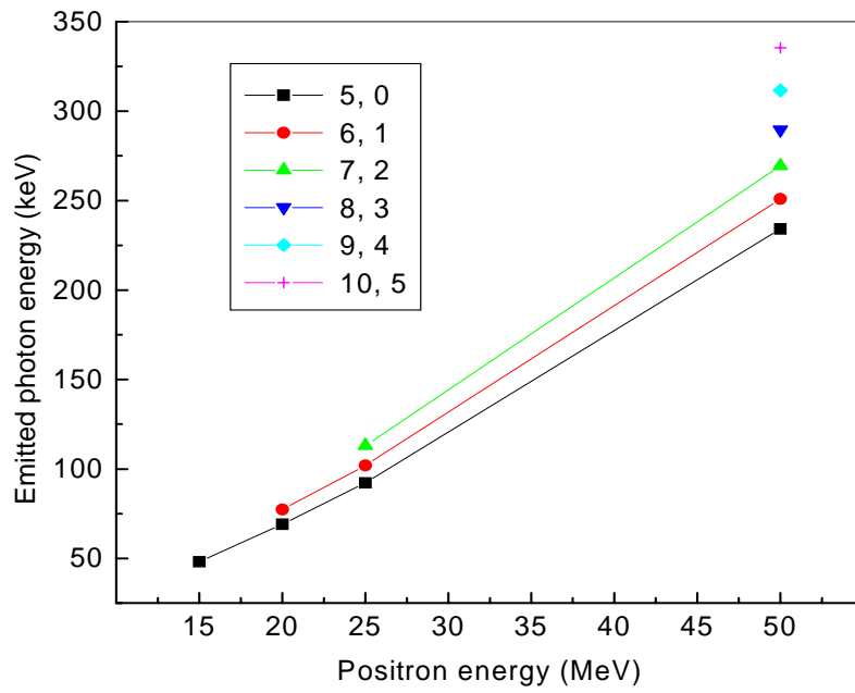
Fig. (3): The emitted photon energy in the forward direction due to n,n-5 transitions between higher quantum states of transverse motion in the planar direction (100) in copper as a function of positron energy up to 50 MeV.
